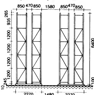
⑩ Section through pallet rack for stacker loading. U-section steel guide rails for stackers
